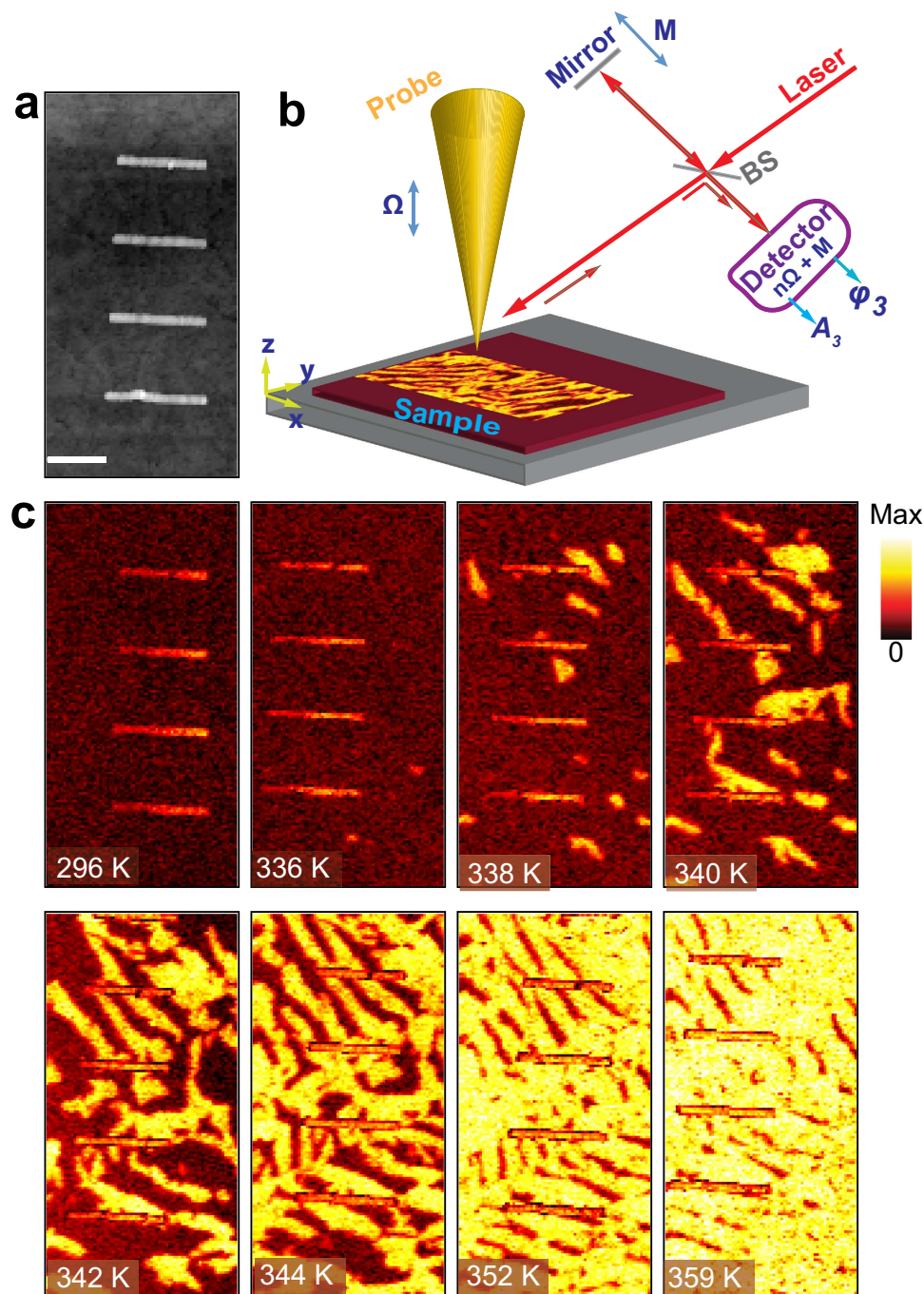
Figure 1. Temperature dependent nanoscale near-field amplitude images of IMT emergence and progress around the infrared antennas. (a) Topography of the four antennas on VO 2 film. The scale bar indicates 1 \mu\text{m} . (b) Schematic of the s-SNOM experimental setup, which allows polarization-controlled simultaneous imaging of IR plasmonic antenna modes together with the phase spatial evolution of VO 2 phase transition in amplitude and phase. The coordinate system is positioned so that the y axis is directed along nanorods and the z-axis is normal to the plane of the nanostructure. (c) Temperature-dependent near-field amplitude images reveal IMT via forming initial metallic nanodomains, which grow and connect to stripes and quasi-uniform metallic phase.
