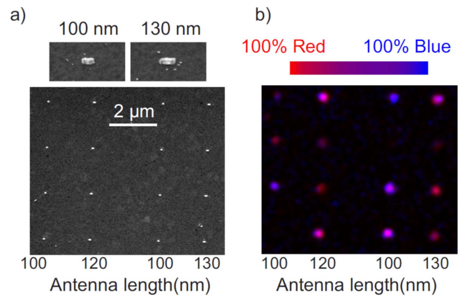
Figure 21. Spectrally selective SH imaging. (a) SEM images of an array of Au nanoantennas of different lengths and zoom-in on individual 100 nm and 130 nm nanoantennas. (b) Two-colour SH image of the same array, showing contrast between different NPs, with longer nanoantennas more red. The blue ( \lambda < 400 nm) and red ( 400 < \lambda < 420 nm) side of the SH-spectrum are pseudo-coloured blue and red. Reprinted from [172], with the permission of AIP Publishing.
