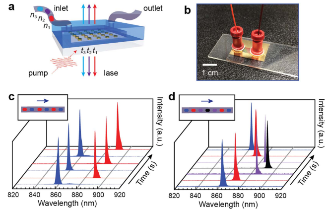
Figure 19. Real-time tunable lasing emissions from gold NP arrays. (a) Scheme of dynamic nanolaser. (b) Optical micrograph of device. (c) Real-time switching between two lasing wavelengths and (d) four lasing wavelengths.
