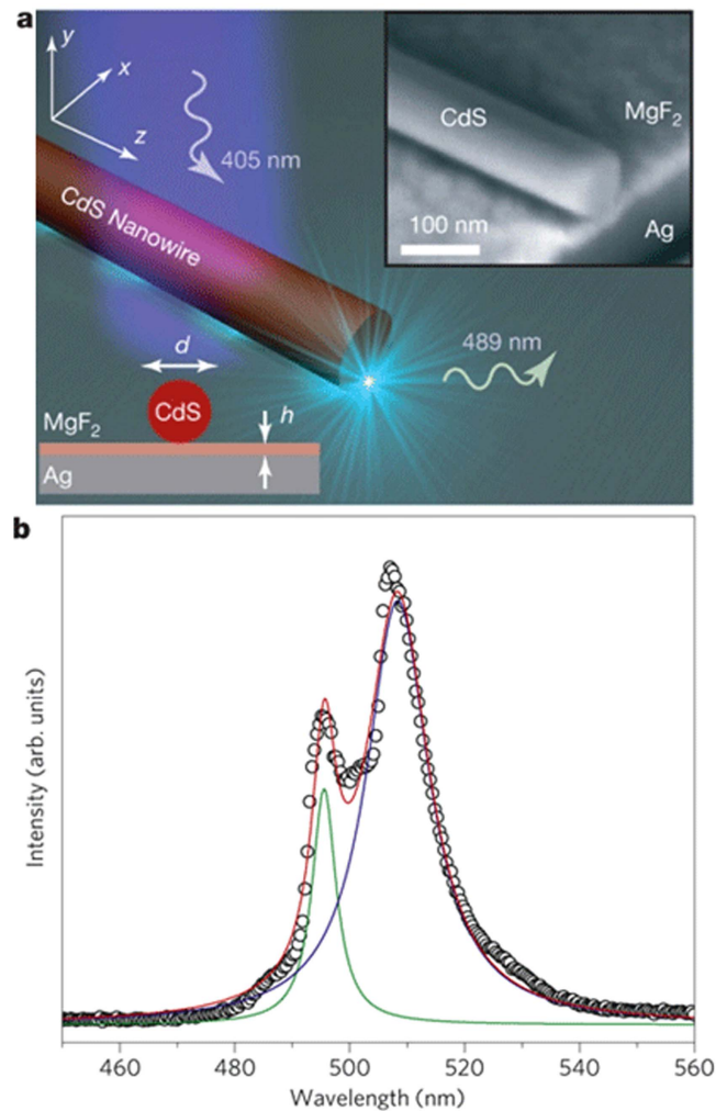
Figure 16. The hybrid plasmon laser concept and demonstration. (a) The laser design with CdS-MgF 2 -Ag configuration. (b) Room temperature plasmon nanolaser enabled by total internal reflections, as evidenced by the fact that cavity modes are observed even in spontaneous emission spectrum indicating excellent cavity feedbacks. Experimental data are well fitted (red curve) by convolution of two calculated cavity modes (green: 495.5 nm; blue: 508.4 nm).
