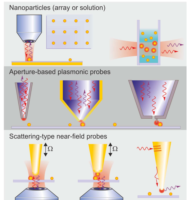
Figure 9. Schematic overview of plasmon-based approaches to light localization and nanoscopy.
