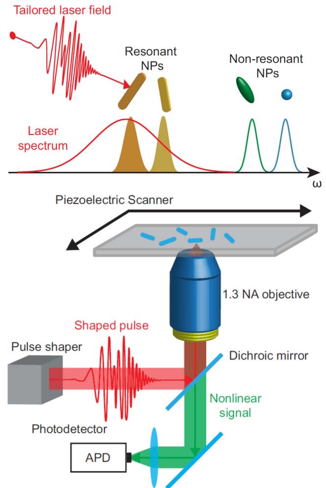
Figure 20. (Top) A broadband ultrashort laser pulse interacts with nanoparticles (NPs). By fabricating nanostructures in resonance with the laser spectrum, tailored laser fields can actively control light–matter interactions in resonant NPs. (Bottom) The phase-shaped laser beam excites a NP in a diffraction-limited spot. The non-linear signal of the NP is collected by a high-NA objective and detected on a photon counting avalanche photodiode (APD).
