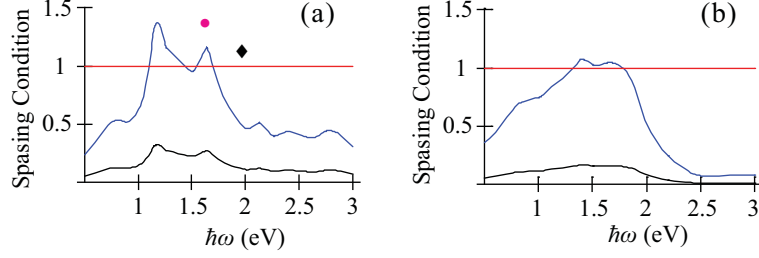
Fig. 6. Spasing criterion as a function of optical frequency \omega . The straight line (red on line) represents the threshold for the spasing and full loss compensation, which take place for the curve segments above it. (a) Computations for silver. The chromophore concentration is n_c = 6 \times 10^{18} \text{ cm}^{-3} for the lower curve (black) and n_c = 2.9 \times 10^{19} \text{ cm}^{-3} for the upper curve (blue on line). The black diamond shows the value of the spasing criterion for the conditions of Ref. [48] – see the text. (b) Computations for gold. The chromophore concentration is n_c = 3 \times 10^{19} \text{ cm}^{-3} for the lower curve (black) and n_c = 2 \times 10^{20} \text{ cm}^{-3} for the upper curve (blue on line).
