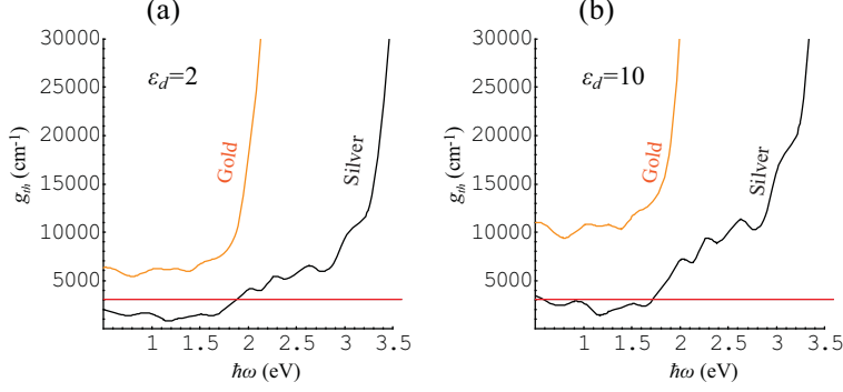
Fig. 3. Threshold gain for spasing g_{th} for silver and gold, as indicated in the graphs, as a function of the spasing frequency \omega . The red line separates the area g_{th} < 3 \times 10^3 \text{ cm}^{-1} , which can relatively easily be achieved with direct band-gap semiconductors (DBGSSs). The real part of the gain medium permittivity is denoted in the corresponding panels as \epsilon_d .
