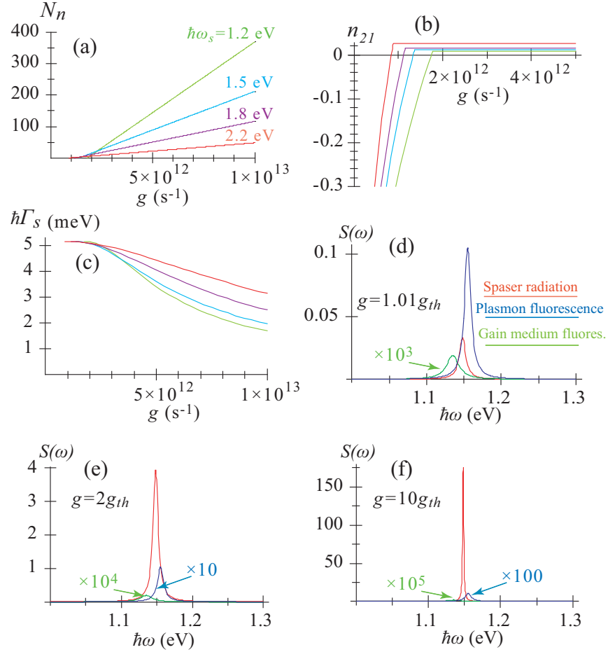
Fig. 4. Spaser SP population and spectral characteristics in the stationary state. The computations are done for a silver nanoshell with the external radius R_2 = 12 nm; the detuning of the gain medium from the spasing SP mode is \hbar(\omega_{21} - \omega_n) = -0.02 eV. The other parameters are indicated in the text in Sec. 3.2. (a) Number N_n of plasmons per spasing mode as a function of the excitation rate g (per one chromophore of the gain medium). Computations are done for the dipole eigenmode with the spasing frequencies \omega_s as indicated, which were chosen by the corresponding adjustment of the nanoshell aspect ratio. (b) Population inversion n_{12} as a function of the pumping rate g . The color coding of the lines is the same as in panel (a). (c) The spectral width \Gamma_s of the spasing line (expressed as \hbar\Gamma_s in meV) as a function of the pumping rate g . The color coding of the lines is the same as in panel (a). (d)-(f) Spectra of the spaser for the pumping rates g expressed in the units of the threshold rate g_{th} , as indicated in the panels. The curves are color coded and scaled as indicated.
