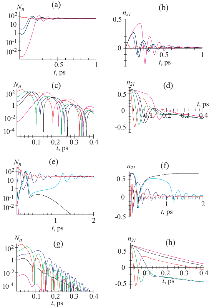
Fig. 5. Ultrafast dynamics of spaser. (a) For monostable spaser (without a saturable absorber), dependence of SP population in the spasing mode N_n on time t . The spaser is stationary pumped at a rate of g = 5 \times 10^{12} \text{ s}^{-1} . The color-coded curves correspond to the initial conditions with the different initial SP populations, as shown in the graphs. (b) The same as (a) but for the temporal behavior of the population inversion n_{21} . (c) Dynamics of a monostable spaser (no saturable absorber) with the pulse pumping described as the initial inversion n_{21} = 0.65 . Coherent SP population N_n is displayed as a function of time t . Different initial populations are indicated by color-coded curves. (d) The same as (c) but for the corresponding population inversion n_{21} . (e) The same as (a) but for bistable spaser with the saturable absorber in concentration n_a = 0.66n_c . (f) The same as (b) but for the bistable spaser. (g) The same as (e) but for the pulse pumping with the initial inversion n_{21} = 0.65 . (h) The same as (g) but for the corresponding population inversion n_{21} .
